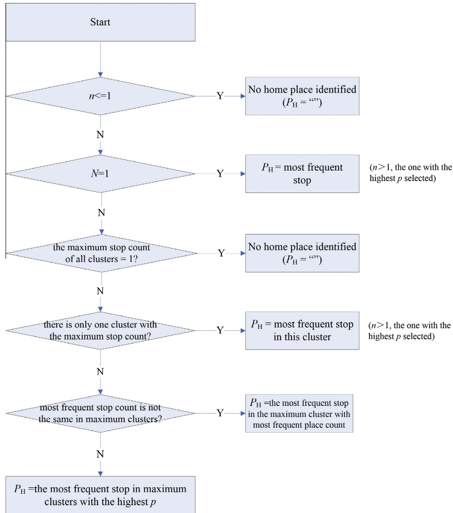
Fig. 6. Decision tree diagram for identifying home locations based on one-day results. Note that n is the count of home locations identified for a cardholder during a week, N is the count of clusters of the cardholder, and P_H is an imputed home location for this cardholder. p is the potential of a home location.
